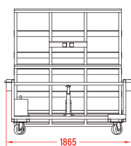
Standard trolley
