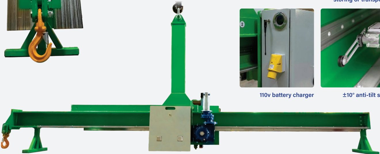
The stand helps to protect the overhang beam when storing or transporting
