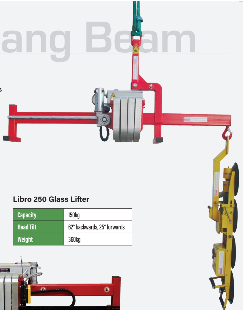
Libro 250 Compact Overhang Beam
