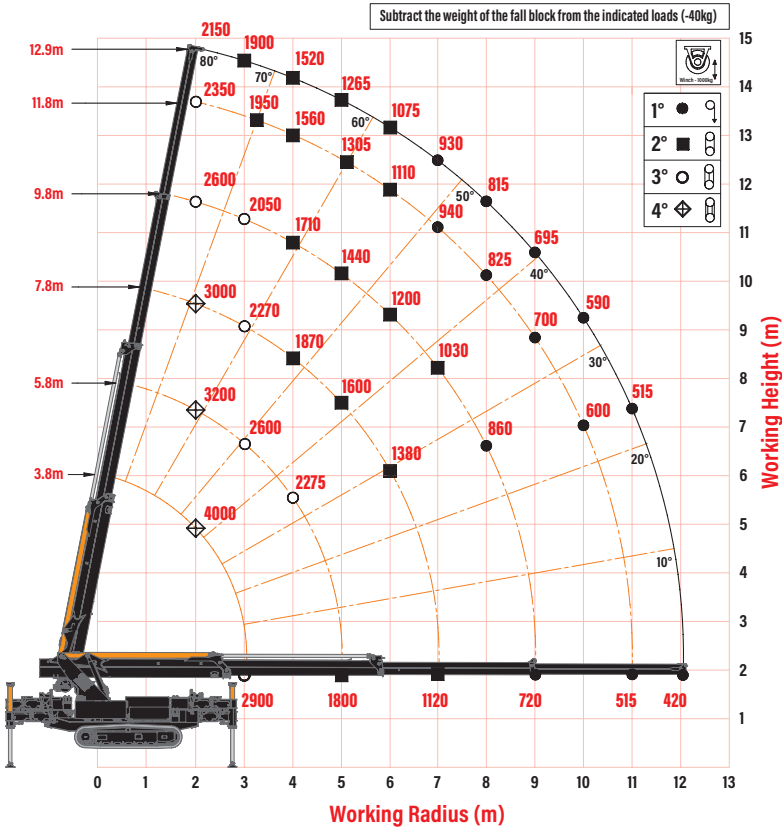
Crane Capacity With Winch - Rated Loads (kg)
