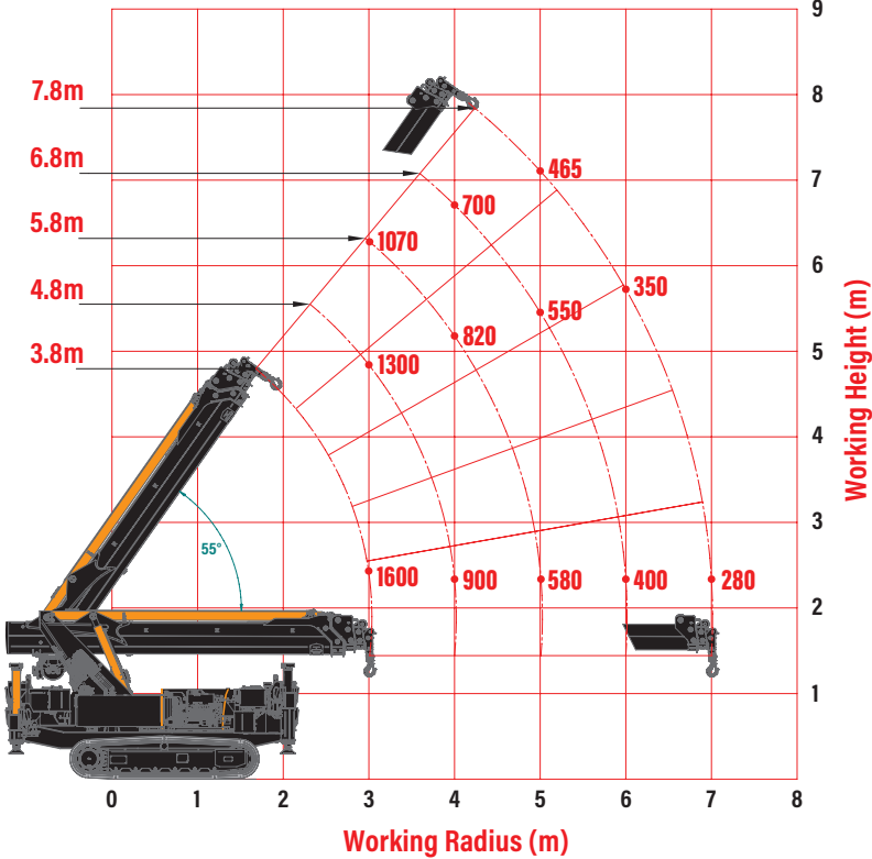
Pick & Carry - Rated Loads (kg)
