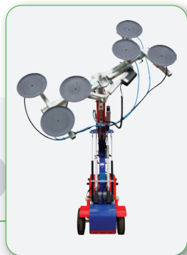
Optional 90° powered rotation kit Reference Code: GRG0985
