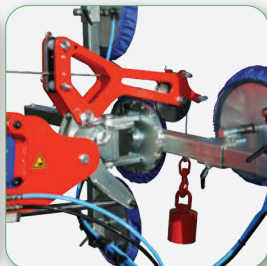
Optional electric winch version available (500kg)
