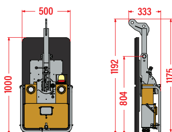
Vertical Wall Panels - With Long Arm
