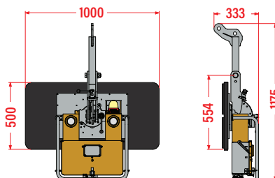
Horizontal Wall Panels - With Long Arm
