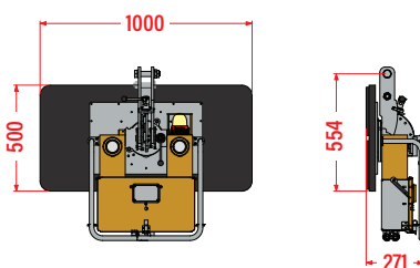
Horizontal Wall Panels - With Short Arm
