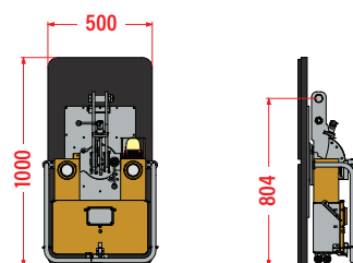
Vertical Wall Panels - With Short Arm
