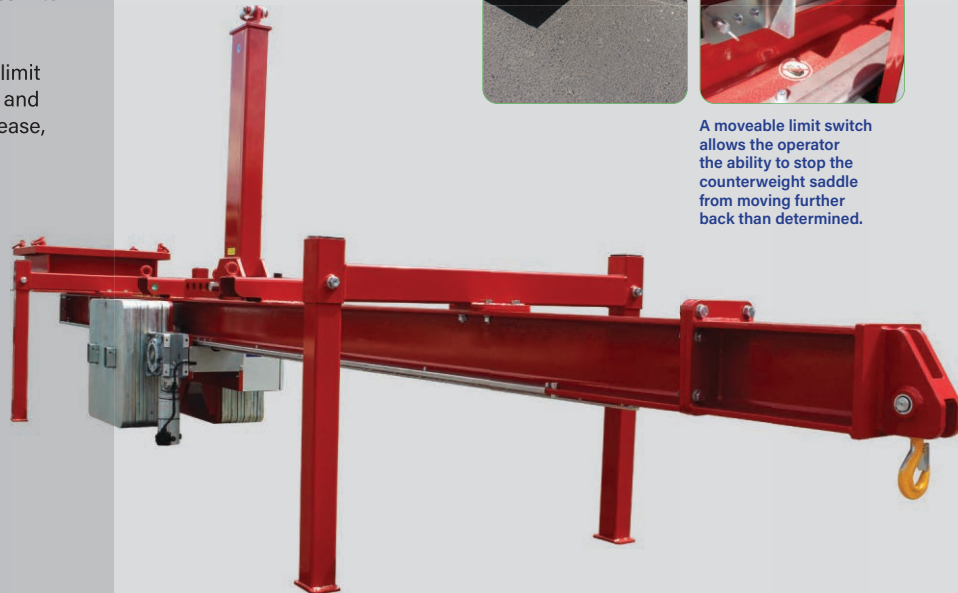
Featuring a removable counterweight, note the counterweight must be installed when using the corner lifter attachment. (Weight of removable counterweight: approx. 1500kg)
