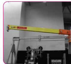
Optional 1.2m long jib (150kg capacity)
